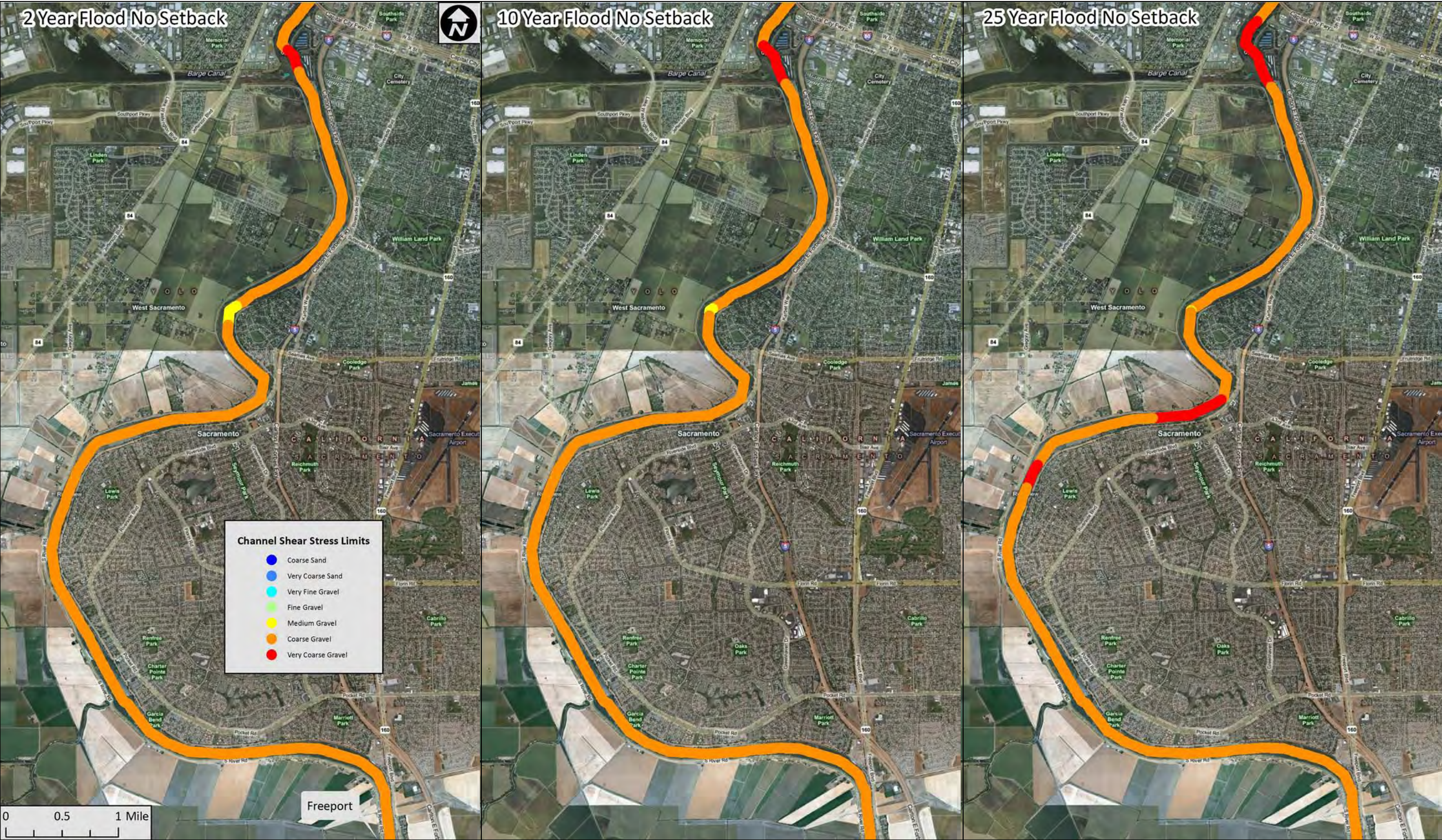
Shear stress limits based on Fischenich, 2001. Colors represent upper limit of shear stress power. Orthoimagery courtesy of Bing Maps. cbec eco engineering Historic and Current Preliminary Geomorphic Assessment- Southport EIP Absolute Channel Shear Stress Existing- I Project No. 11-1003 Created By: WGW Figure 4-7
