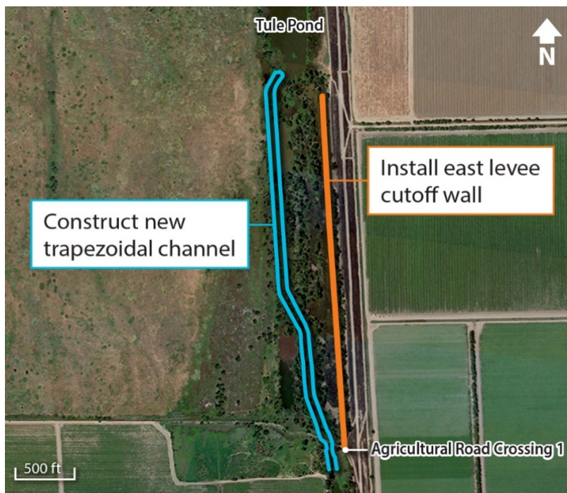
Figure 8. Tule Channel alignment, Agricultural Road Crossing 1 Locations
