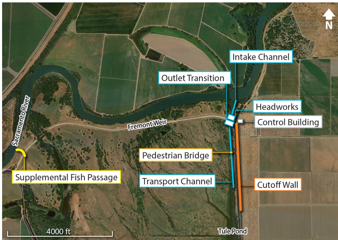
Figure 7. Project Feature Locations- North of Tule Pond
