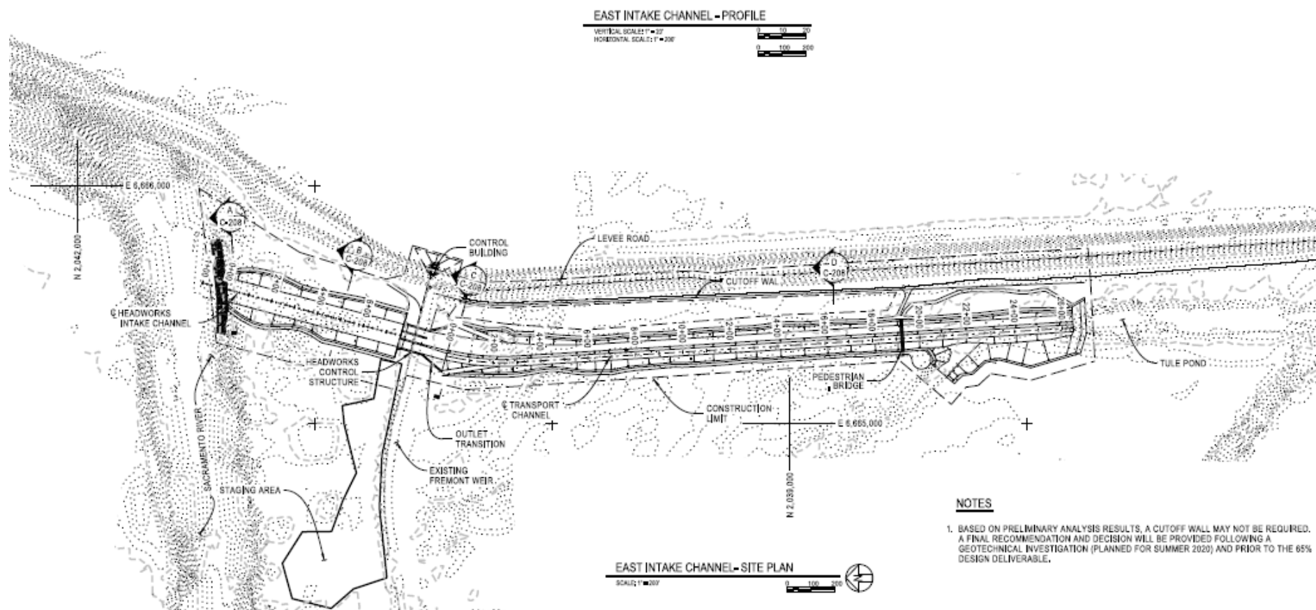
Figure 9. Intake Channel, Headworks Structure, Outlet Transition, Transport Channel
