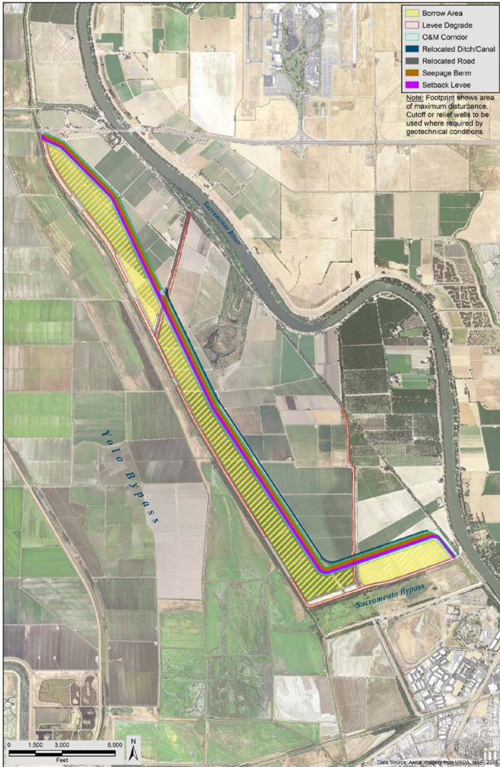
Figure 3. Alternative 2 – 7-mile Setback Partial Degrade (DWR’s Preferred Alternative)
