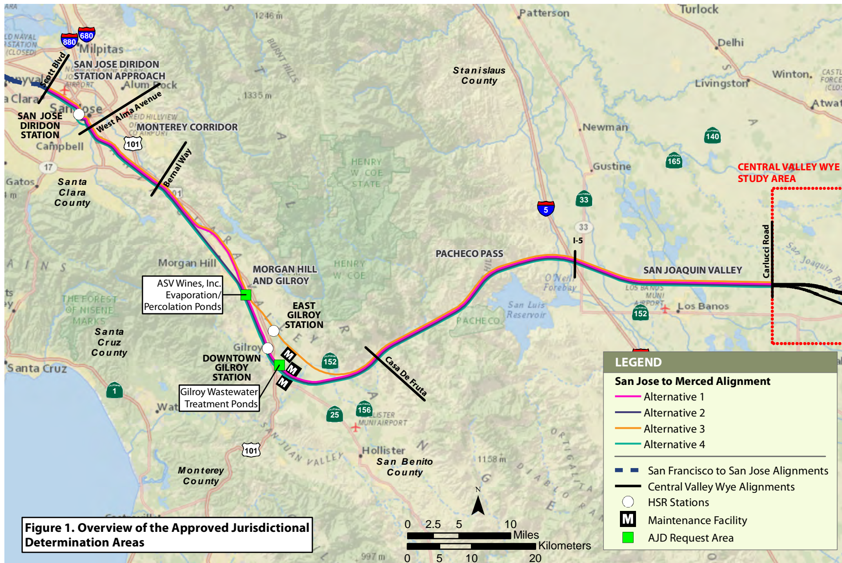
San Jose to Merced Section of the California High Speed Rail Project - June 2019
