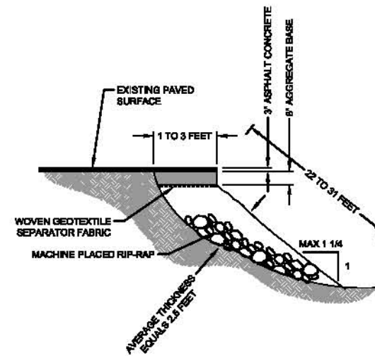
TYPICAL SLOPE REPAIR SECTION FOR CENTRAL SITE NOT TO SCALE
