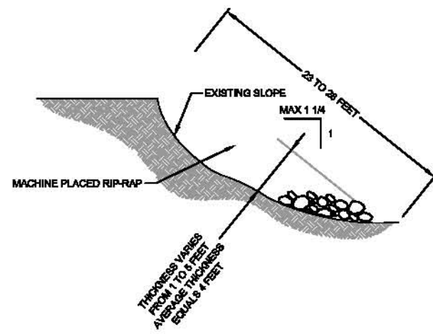
TYPICAL SLOPE REPAIR SECTION FOR EASTERN SITE NOT TO SCALE
