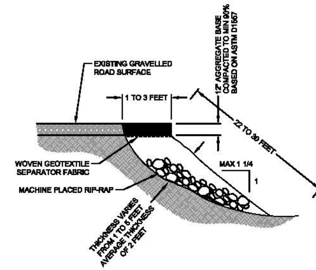
TYPICAL SLOPE REPAIR SECTION NOT TO SCALE
