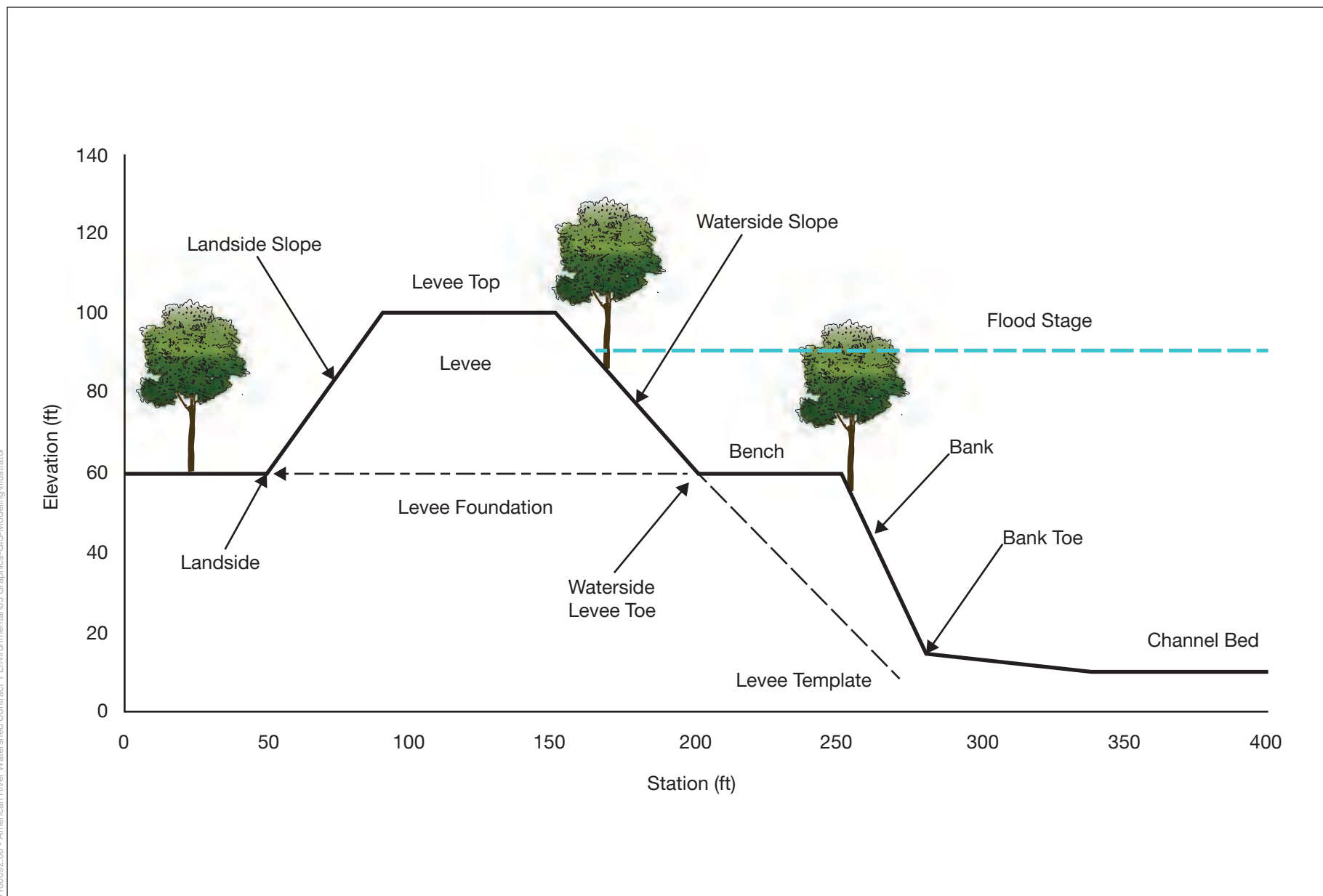
Figure 2-2 Levee Terminology
