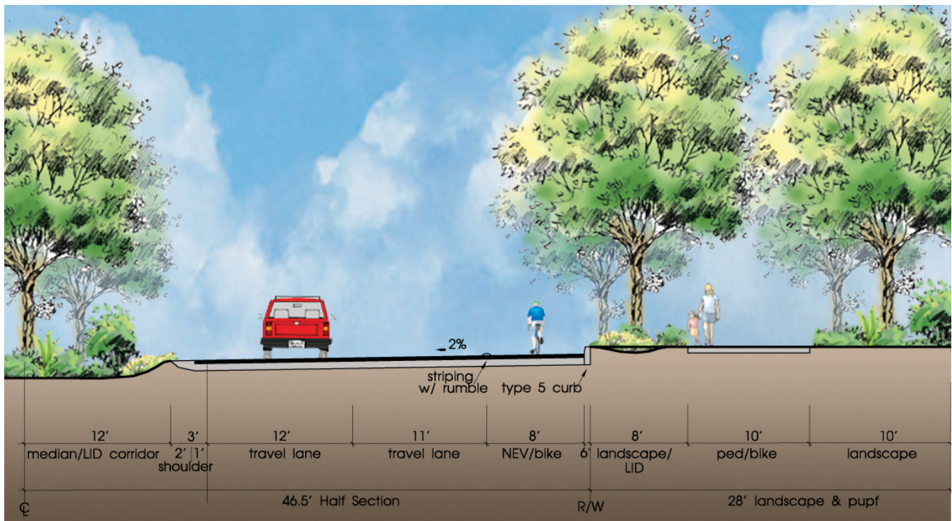
Typical pedestrian trail and bike cross section
